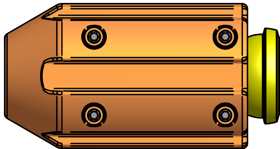
1 X BOP0132C 120 - 108 MULTIPLANE MALE - MALE CABLE CLAMP & CENTRALISER SHELL ASSEMBLY (DETAIL "X")
